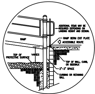
SUGGESTED ELEVATED RAMP BERM EXIT PLATE 24" PLUS DECK TO GRADE/DB INSTALLATION REFER TO RAMP BERM EXIT PLATE INSTALLATION SHEET SEE PLAN FOR ELEVATION OF PLATE
