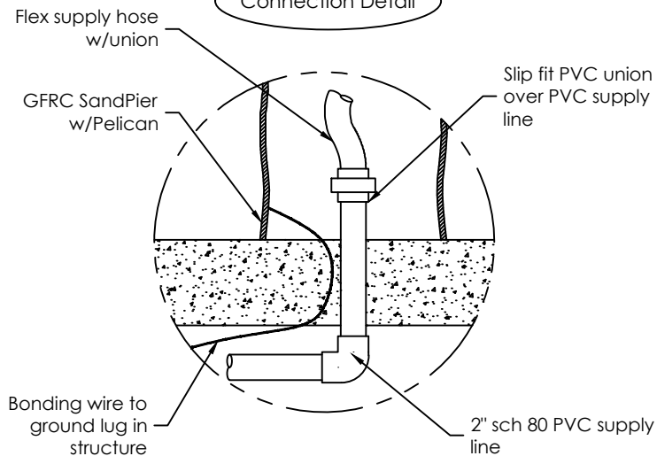
Connection Detail
