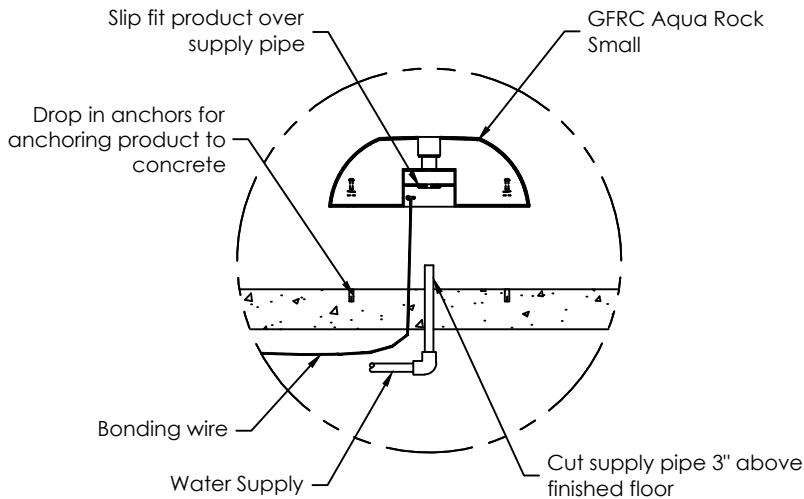
Connection Detail
