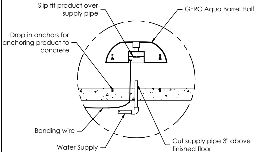
Connection Detail
