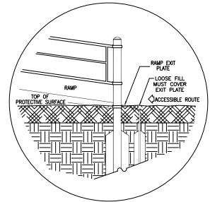
SUGGESTED RAMP EXIT PLATE 8"/12" DECK TO GRADE LOOSE FILL / DB / 12" SURFACE MOUNT INSTALLATION REFER TO RAMP EXIT PLATE INSTALLATION SHEET
