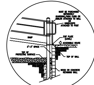
SUGGESTED ELEVATED RAMP EXIT INSTALLATION RAMP ELEVATION TO BE 6\"/>
