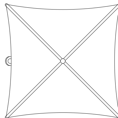
237672 SKYWAYS 10' X 10' CANTILEVER SINGLE POST PYRAMID W/14' ENTRANCE
