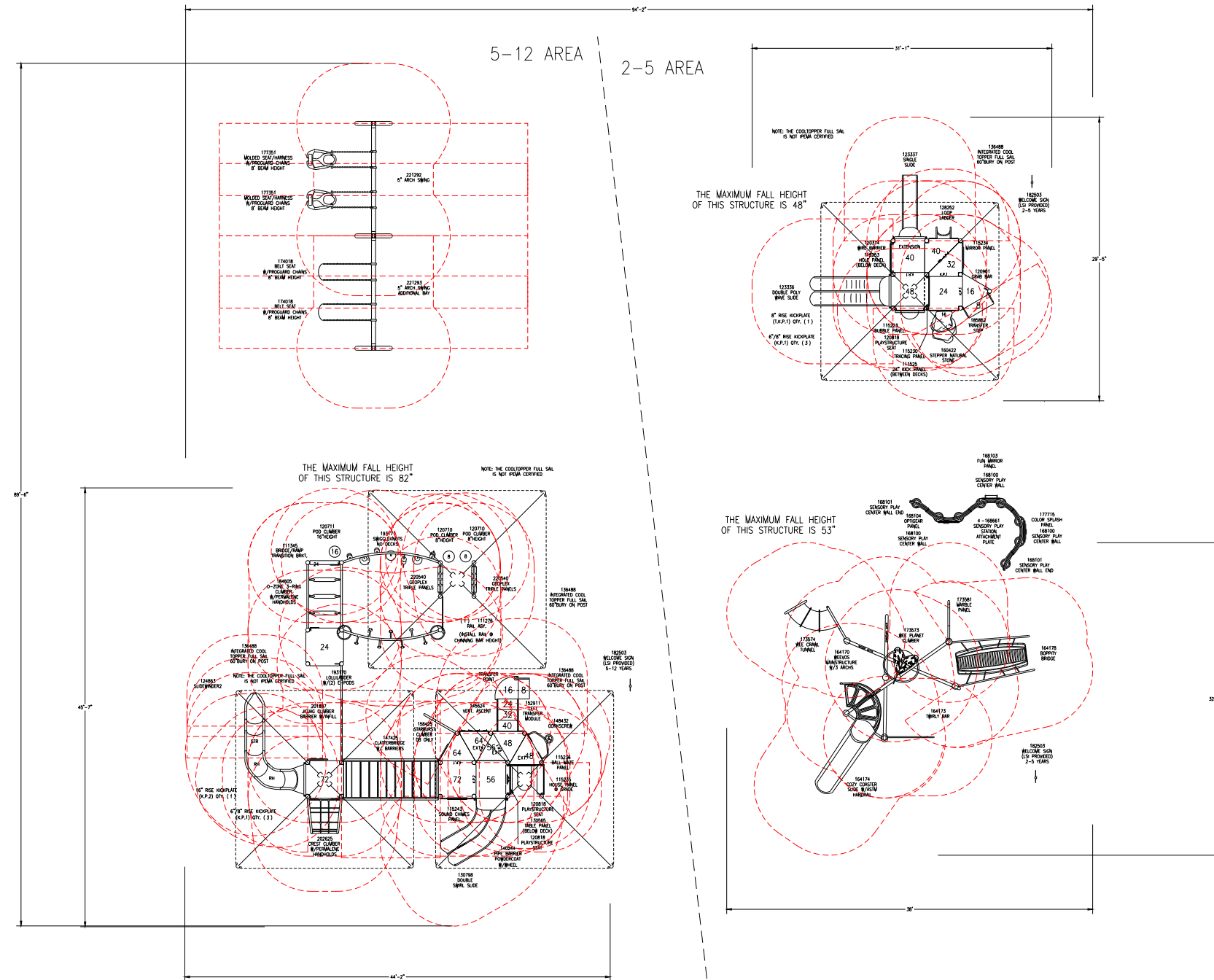
2-5 AREA PlayBooster® (2-5 years) Max Fall Height: 48 inches Weevos® (2-5 years) Max Fall Height: 53 inches
