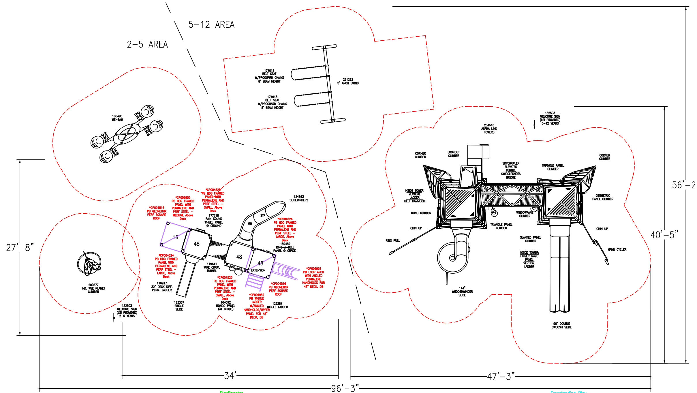
2-5 AREA (STRUCTURE DOES NOT MEET ADA) PlayBooster (2-5 years) Max Fall Height: 48 inches
